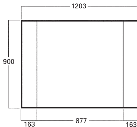
GRAPHIC SIZE
