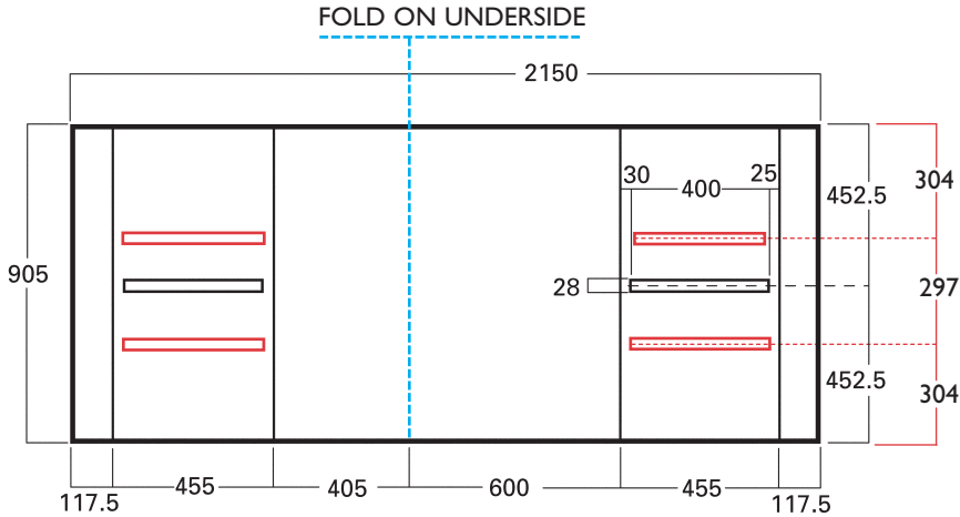
GRAPHIC SIZE FOR ONE AND TWO SHELF UNIT
